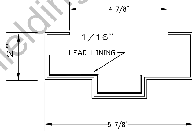
16GA FRAME SECTION DETAIL
